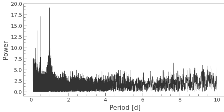
Figure 3: Periodogram of the residuals, showing a peak at a period of 1 d.
