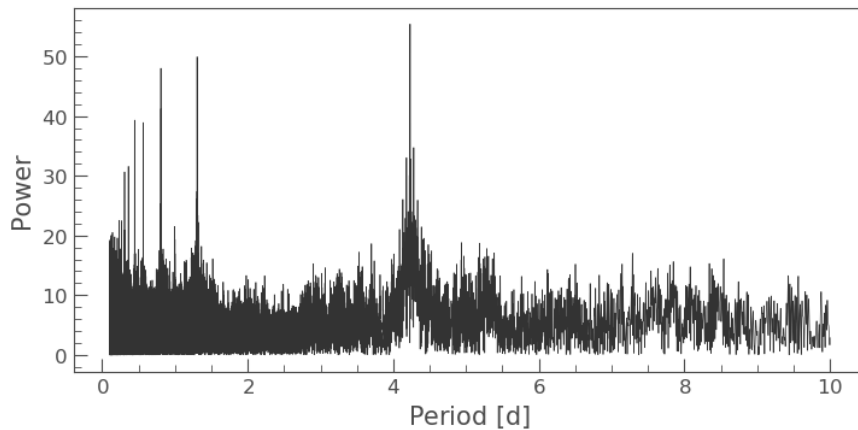
Figure 1: LOMB-SCARGLE periodogram of the original 51 Peg data, showing a peak at a period of 4.23 d.
