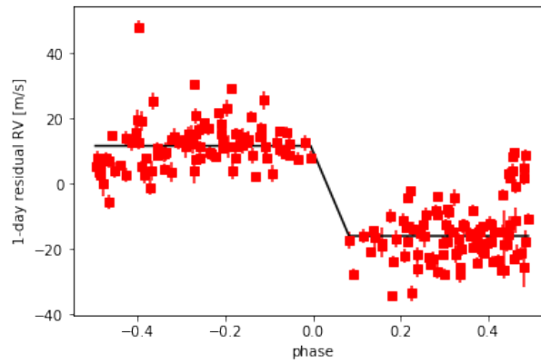
Figure 4: Intra-day residuals, showing a calibration offset between two different observing locations.
