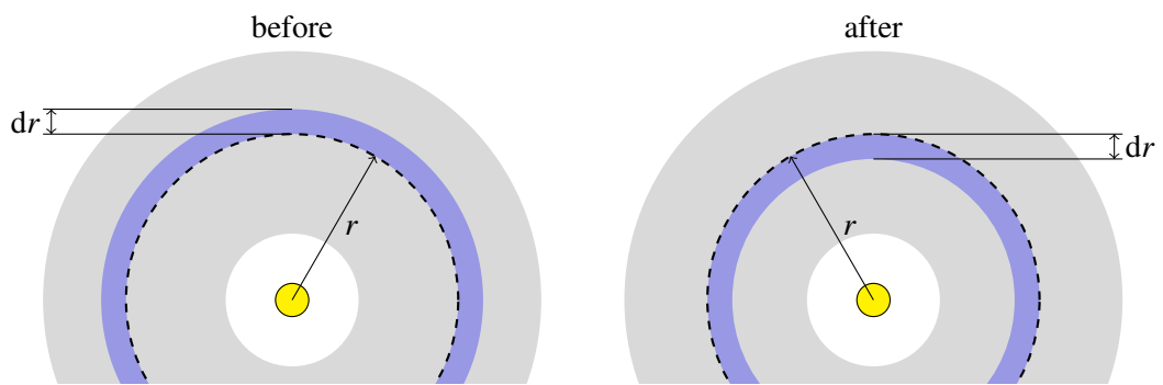
Figure 5: A narrow annulus of width dr drifts inwards, passing the dashed line that marks a distance of r .
